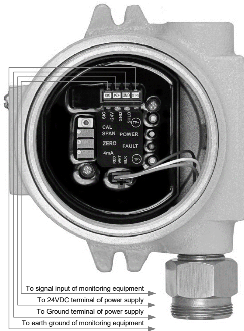
Figure 2: Wiring diagram
