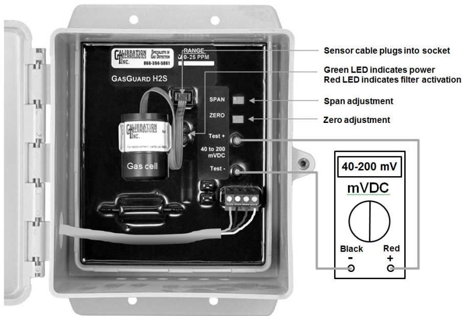
Figure 3: Sensor board components and zero/span adjustments
