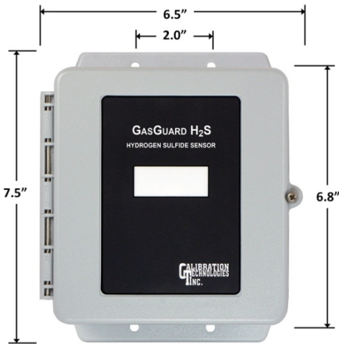
Figure 1: Mounting dimensions
