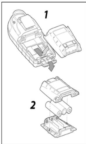
Figure 1: Replacing the Batteries
