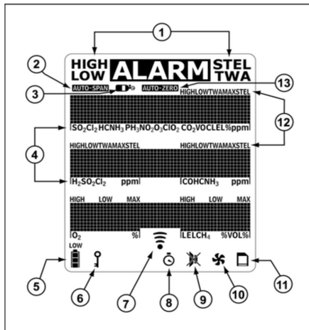
Figure 2. Screen Elements
