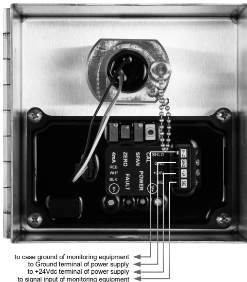
Figure 3: Wiring diagram
