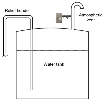
Figure 2: Discharge to Diffusion Tank
